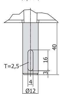
Round shaft with feather key (Option)
